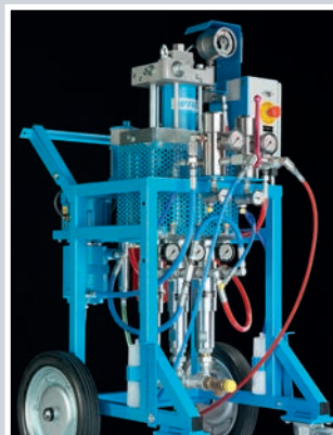
WIWA POWERPACK 2K hydraulic systems
